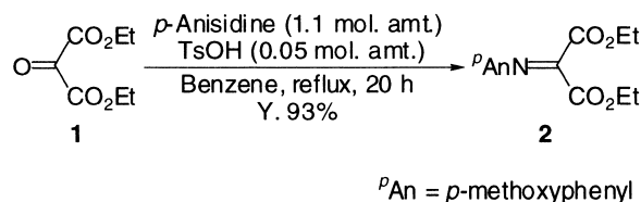
Scheme 1. Preparation of iminomalonate.
