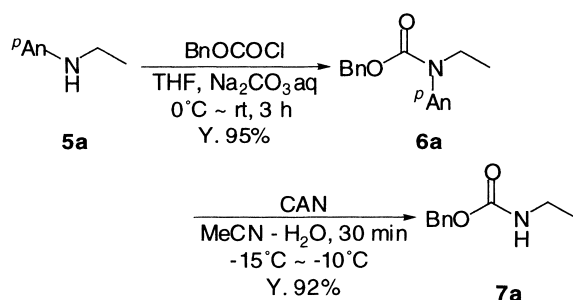
Scheme 4. Removal of p -methoxyphenyl group.
