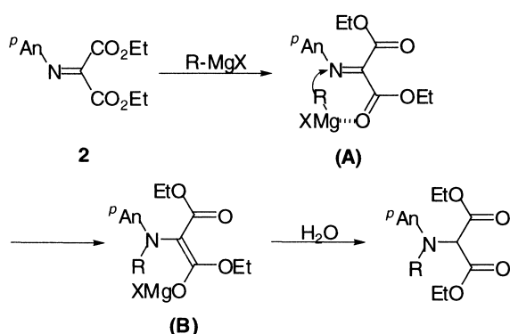
Scheme 2. Mechanism of the amination reaction.
