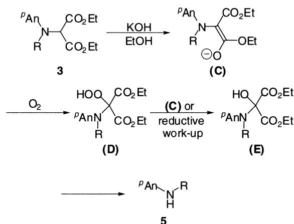
Scheme 3. Mechanism of the oxidative cleavage.
